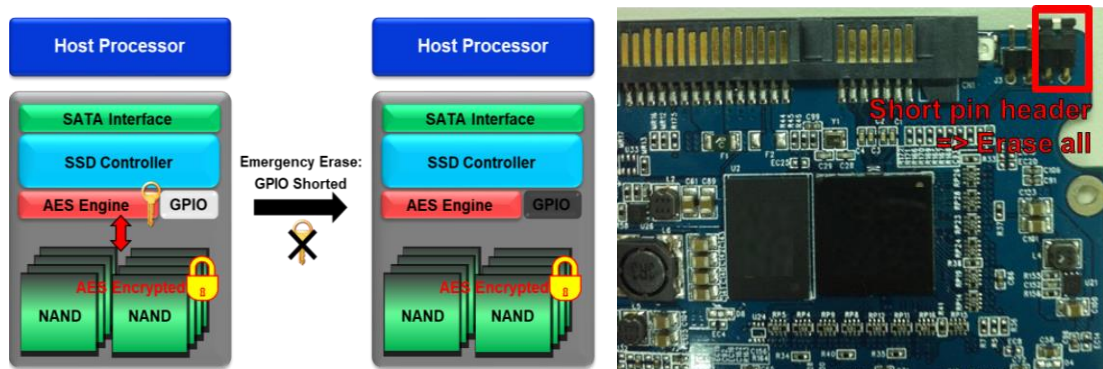
Figure 12: a) Principle of Emergency Erase; Emergency Erase
