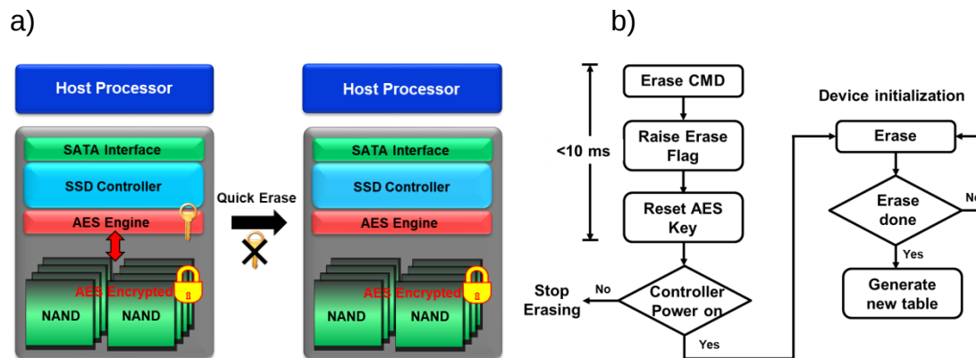
Figure 10: a) Principle of Quick Erase; b) Process of Quick Erase
